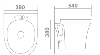
RIMLESS MILAN WALL HUNG TOILET 71-6480 54 X 38 X 38 White 71-6481 54 X 38 X 38 Ivory
