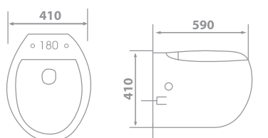
MONILA WALL HUNG TOILET 71-6500 59 X 41 X 41 White 71-6501 59 X 41 X 41 Ivory
