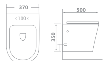
RIMLESS VIENNA WALL HUNG TOILET 71-6490 50 X 37 X 35 White 71-6491 50 X 37 X 35 Ivory
