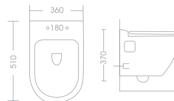
DOVICA WALL HUNG TOILET 71-6520 51 X 36 X 37 White
