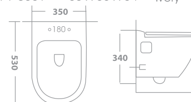
CHENAL WALL HUNG TOILET 71-6550 53 X 35 X 34 White 71-6551 53 X 35 X 34 Ivory
