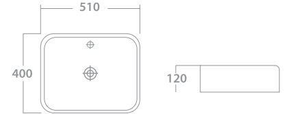
ABOVE COUNTER SINK 71-5440 51 X 40 X 12 White
