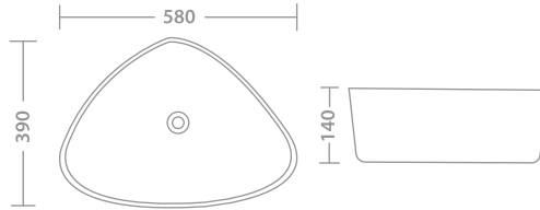
ABOVE COUNTER SINK 71-5470 58 X 39 X 14 White
