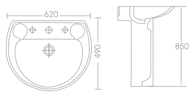
OSLO PEDESTAL SINK BASIN 71-0160 62 X 49 X 85 White 71-0170 62 X 49 X 85 Ivory
