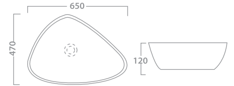
ABOVE COUNTER SINK 71-5480 65 X 47 X 12 White
