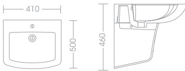
PARCA WALL-MOUNT SINK 71-0785 50 X 41 X 46 White 71-0795 50 X 41 X 46 Ivory
