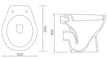
PAN W.C. TOILET 71-6680 46 X 36 White
