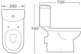
BRAGUE W.C. TOILET 71-6040 70 X 38 X 76 White 71-6041 70 X 38 X 76 Ivory
