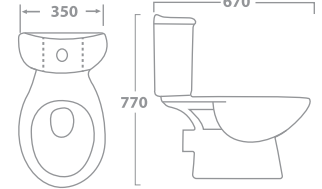
HYGIENE W.C. TOILET 71-6080 67 X 35 X 77 White 71-6081 67 X 35 X 77 Ivory
