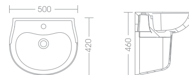
INCI WALL-MOUNT SINK 71-0765 50 X 42 X 46 White 71-0775 50 X 42 X 46 Ivory
