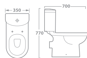
EVEL W.C. TOILET 71-6165 70 X 35 X 77 White 71-6166 70 X 35 X 77 Ivory
