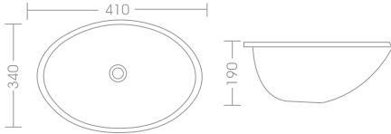
CARVIT ACRYLIC DROP-IN SINK 70-2310 41 X 34 X 19 White 70-2311 41 X 34 X 19 Ivory
