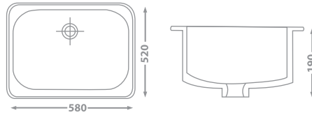
SUPER MARBELLA ACRYLIC KITCHEN SINK 70-2502 58 X 52 X 19 White 70-2512 58 X 52 X 19 Ivory
