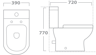
MONTANA W.C. TOILET 71-6020 72 X 39 X 77 White 71-6021 72 X 39 X 77 Ivory
