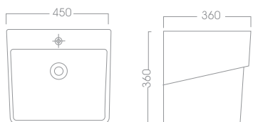
CRYSTAL WALL-MOUNT SINK 71-3255 45 X 36 X 36 White 71-3256 45 X 36 X 36 Ivory
