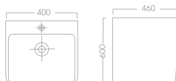
VIVIANA WALL-MOUNT SINK 71-3260 40 X 46 X 60 White 71-3261 40 X 46 X 60 Ivory
