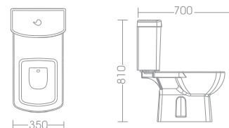
PLAZA W.C. TOILET 71-0721 70 X 35 X 81 White 71-0731 70 X 35 X 81 Ivory
