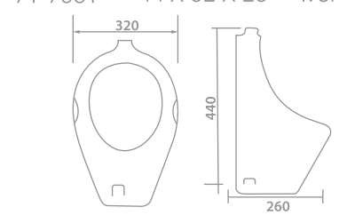
URINAL FLAT BACK URINAL 71-7300 44 X 32 X 26 White 71-7301 44 X 32 X 26 Ivory
