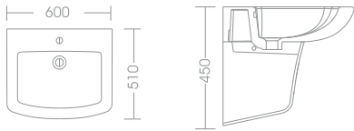
PLAZA WALL-MOUNT SINK 71-0725 60 X 50 X 45 White 71-0735 60 X 50 X 45 Ivory
