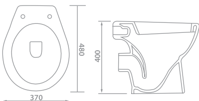
VIVA W.C TOILET 71-6650 48 X 40 X 37 White 71-6651 48 X 40 X 37 Ivory
