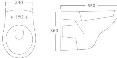
MONIXA WALL HUNG TOILET 71-6440 55 X 36 X 34 White 71-6441 55 X 36 X 34 Ivory
