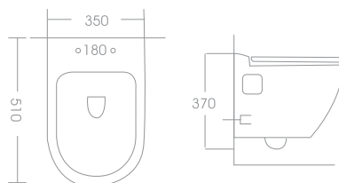
DOMICA WALL HUNG TOILET 71-6510 51 X 35 X 37 White
