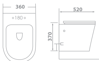
BERLIN WALL HUNG TOILET 71-6530 52 X 36 X 37 White 71-6531 52 X 36 X 37 Ivory
